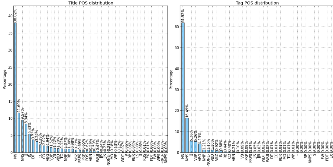
Figure 7.2: Distribution of DeliciousT140 POS categories. Left: title-word POS distribution, right: tag-word POS distribution.
