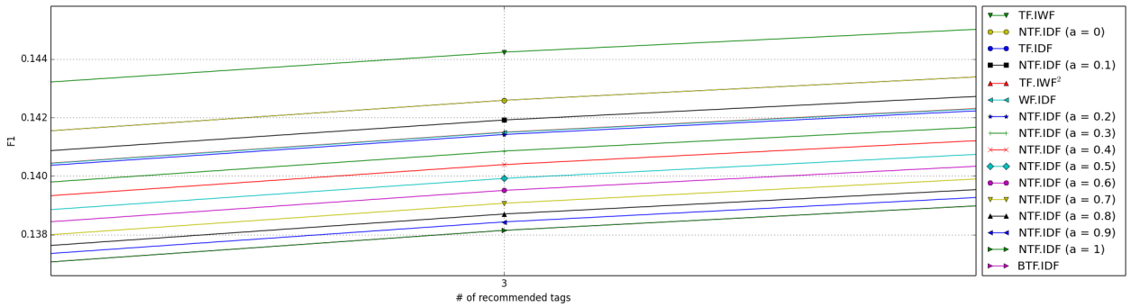
Figure 8.2: DeliciousT140 TF.IDF F1 results zoomed to 3 tags.
