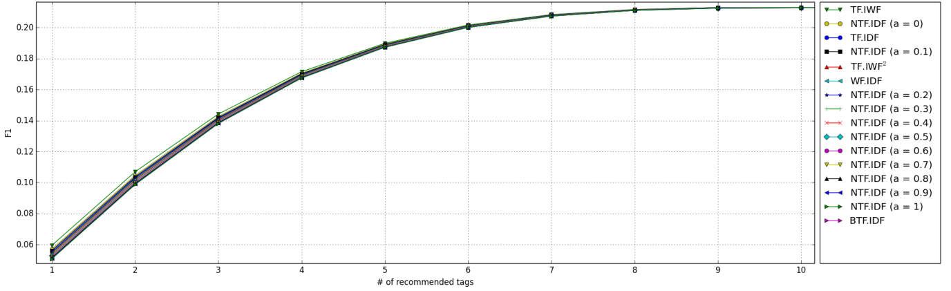
Figure 7.4: DelicousT140 F1 results for TF.IDF & variants
