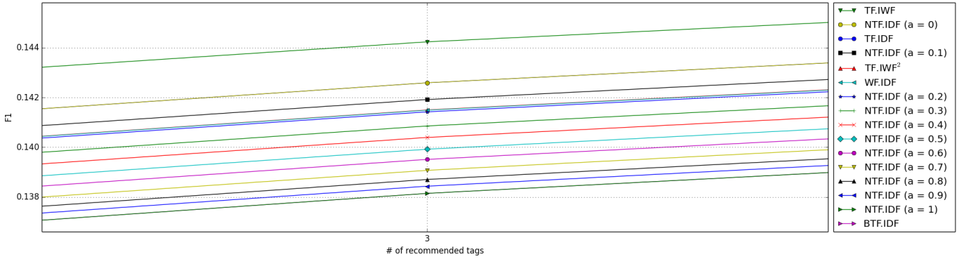
Figure 7.5: DelicousT140 F1 results for TF.IDF & variants
