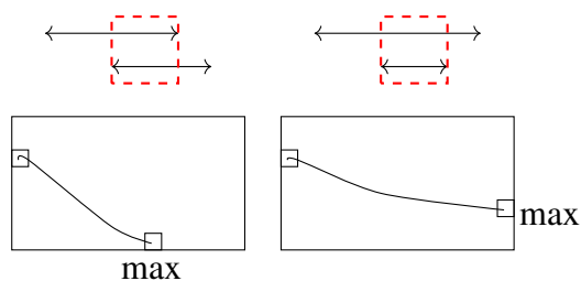
Figure 2: Semi-global alignment: finding overlap or containment.
